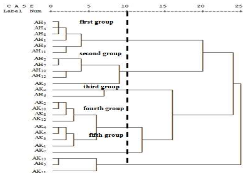
Fig. 1. Dendrogram of pistachio cvs Akbari and Ahmad-Aghaii based on studied traits by Ward method.
