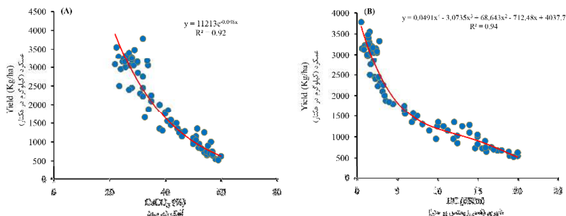
Fig. 1. The best extracted relationship between yield and \text{CaCO}_3 (A) and soil salinity (B)
