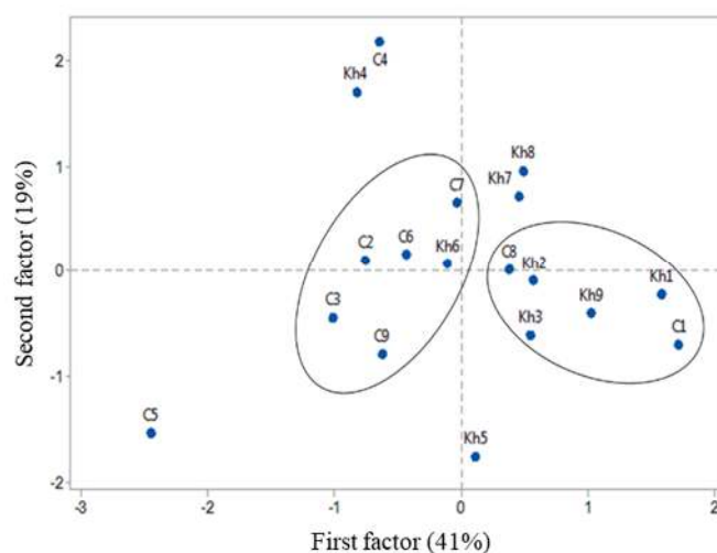
Fig. 6. Score plot for each observation.
