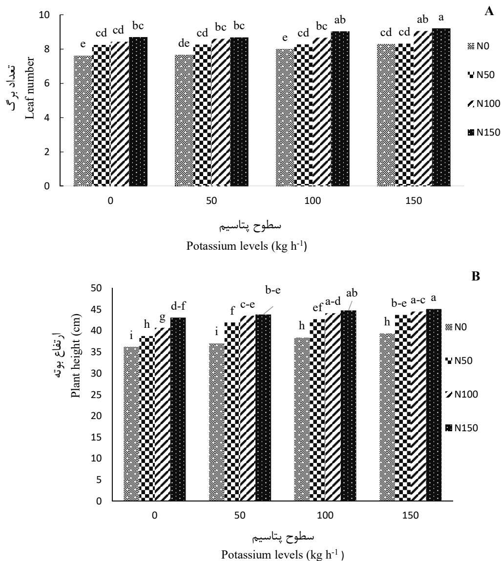
Fig 2. The interaction effect of nitrogen (0, 50, 100 and 150 \text{kg ha}^{-1} ) and potassium (0, 50, 100 and 150 \text{kg ha}^{-1} ) on leaf number (A) and plant height (B) of sweet fennel. In each column, there is no significant difference between treatments with same letters at P \leq 0.05 .
