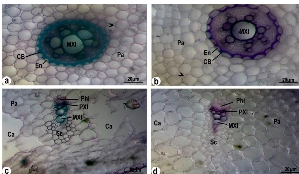
Fig. 4. Mxl metaxyl, Pxl protoxyl, En endoderm, CB Caspari band, Pa parenchyma, Phl phloem, Sc sclerenchyma, Ca air cavity.
