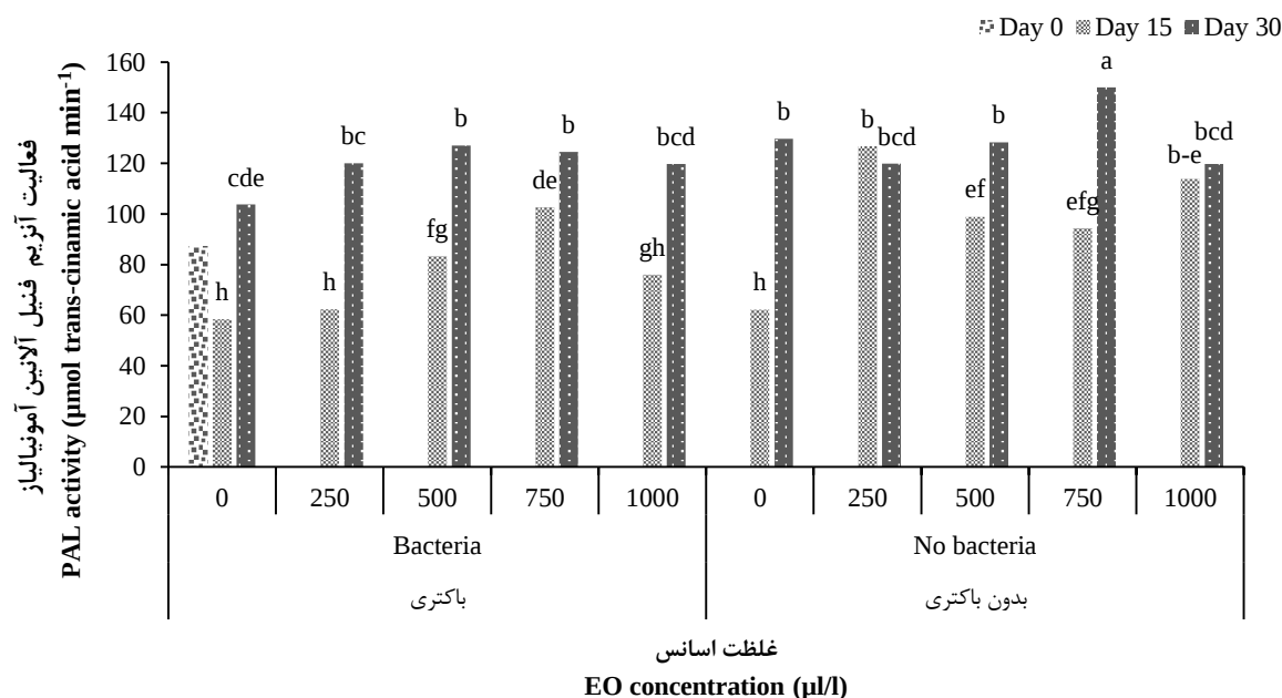
Fig. 5. Interaction effect of oregano essential oil and Bacillus subtilis on the PAL enzyme activity of sweet cherry stored for 30 days at 0\pm1^{\circ}\text{C} with 90–95% relative humidity. Non identical letters indicate a significant difference 5% probability level between means with Duncan test.
