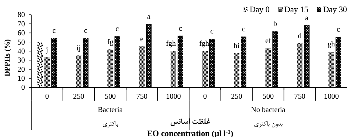
Fig. 3. Interaction effect of oregano essential oil and Bacillus subtilis on the antioxidant activity of sweet cherry stored for 30 days at 0\pm1^\circ\text{C} with 90–95% relative humidity. Non identical letters indicate a significant difference 5% probability level between means with Duncan test.
