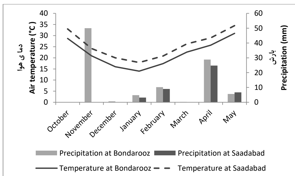
Fig. 1. Air temperature and precipitation in Bondarooz and Saadabad locations.
