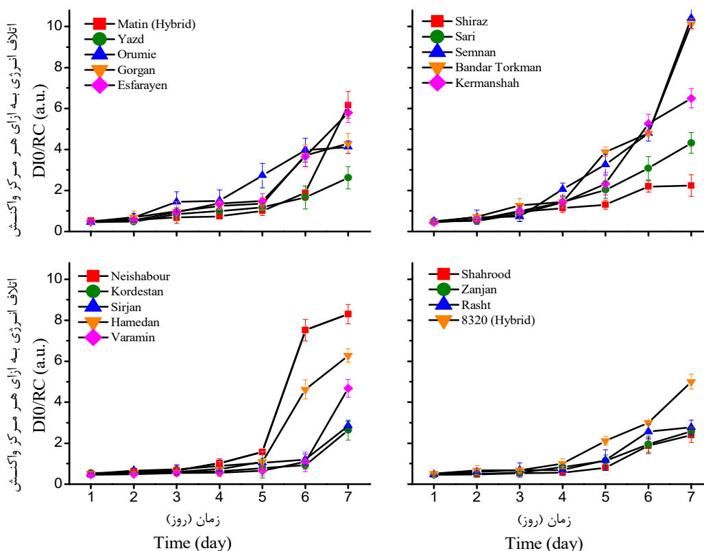
Fig. 5. Changes in the dissipated energy flux per reaction center ( DI_0/RC ) during seven days of water withholding in 17 tomato landraces of Iran and two hybrids. To clarity process, each five landraces placed in one graph (except the bottom right graph).
