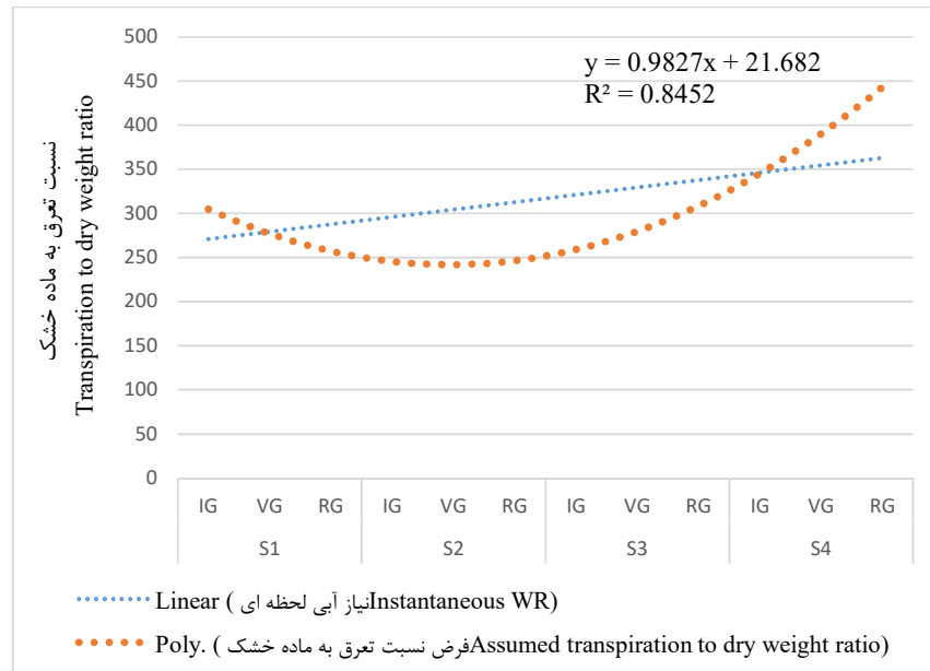
Fig. 2. Regression relationship between instantaneous water requirement and experimental assumption of transpiration ratio to dry weight (S1, S2, S3 and S4) at different stages of initial growth (IG), vegetative growth (VG) and reproductive growth (RG) of greenhouse cucumber in Socrates cultivar (Negin).
